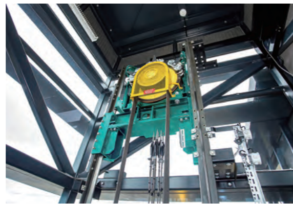
MRL Elevator
